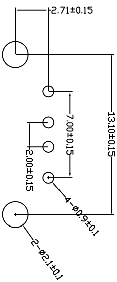
PCB LAYOUT
