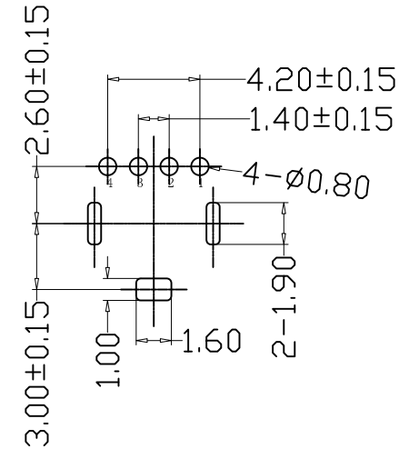
RECOMMENDED PCB LAYOUT GENERAL TOLERANCES: ±0.05
